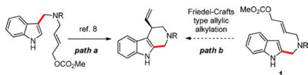
Scheme 1. Different Approaches for the Synthesis of Chiral Tetrahydrocarboline Frameworks
